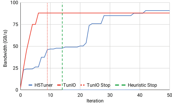
(a) Bandwidth of BD-CATS with TunIO.
