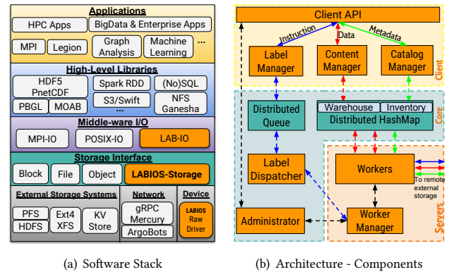
Figure 1: LABIOS overview.
