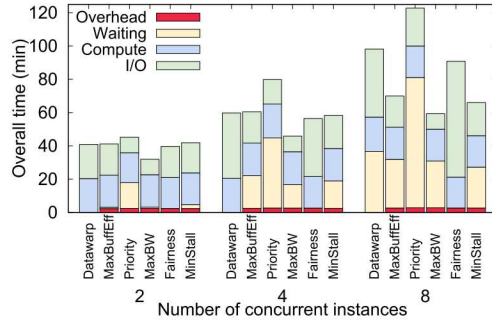
Fig. 6. Execution time and overheads.
