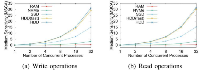
Fig. 2. Sensitivity to Concurrent Access (MSCA).
