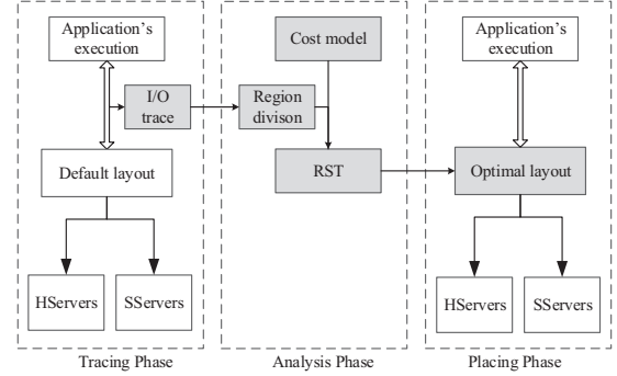
Fig. 3. The procedure for HARL scheme
