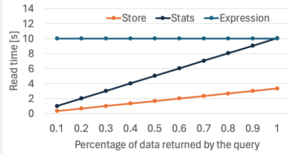
Fig. 7: Read time on Perlmutter for the three strategies when only a percentage of the data is analyzed by readers.
